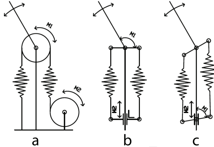
Figure 4: The different possibilities in the class Antagonistic Springs with Independent Motors.
