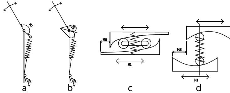
Figure 6: The possibilities in the class Preload Adjustment of Single Spring (a) Maccipa, b) Maccia 2.0, c) VS joint, d) FSJ. )
