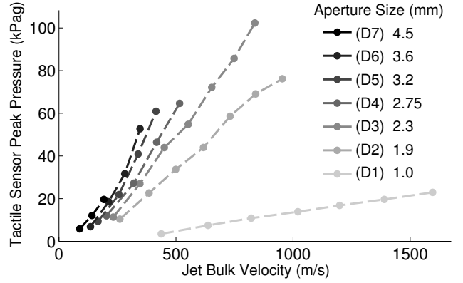
Fig. 4. Peak pressure values obtained from tactile sensor plotted against calculated jet bulk velocity. Each line represents a single aperture size. Traces with fewer points contained peak pressures that were not attainable at the specified aperture size.
