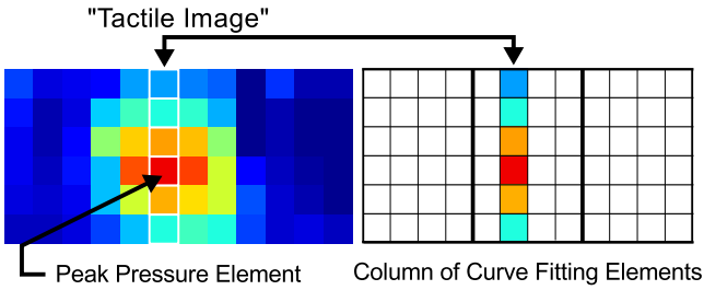
Fig. 3. Tactile data terminology. (Left) Sensor element data was averaged, resulting in a "tactile image" with a peak pressure value. (Right) The peak pressure element determines which column of sensor element values is used for the pressure profile curve fit.
