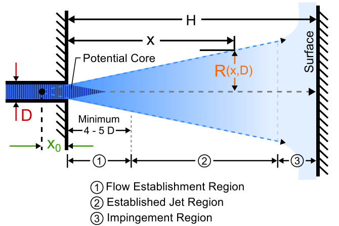
Fig. 2. An ideal round jet develops as a conical shape with a jet spread rate, S . The jet radius ( R ) is a function of the distance from the outlet ( x ) and the aperture diameter ( D ). The jet exhibits properties that can be divided into three distinct regions of interest.
