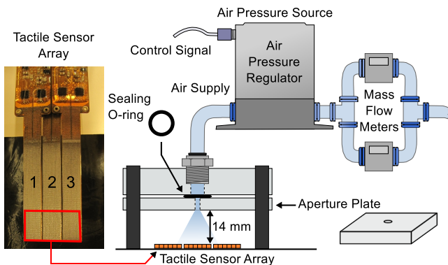
Fig. 1. Setup for tactile sensor and air flow measurements. The air pressure regulator allows pressurized air through the aperture plate and controls supply pressure while mass flow meters record flow rate. An array of capacitive tactile sensors centered under the aperture records distributed pressure as supply pressure and aperture size are varied.
